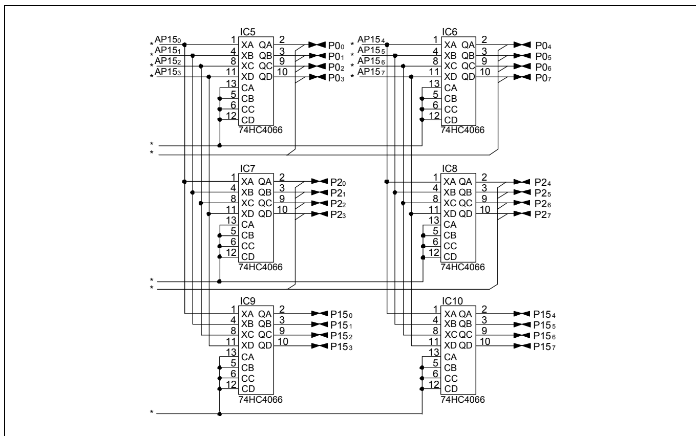
Figure 4.2 Connection diagram (2/2)
